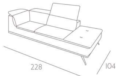
Code 58sx/59dx Corner and terminal chair
